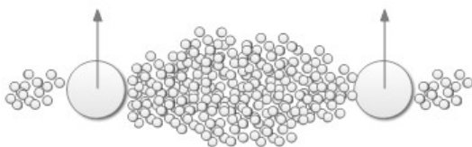
Figure 3.1: Repulsive wall
