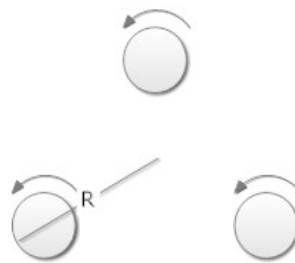
Figure 8.1: Proton
